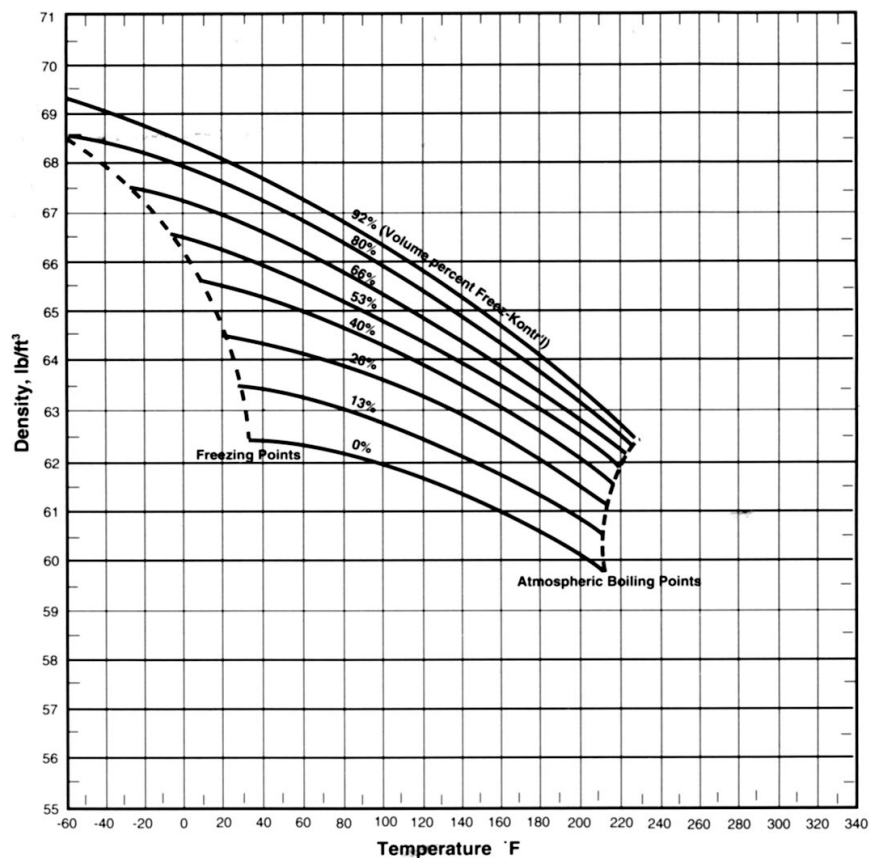
Figure 3 - Densities (lb/ft 3 ) of various solutions of Freez-Kontr'l (percent by volume)
